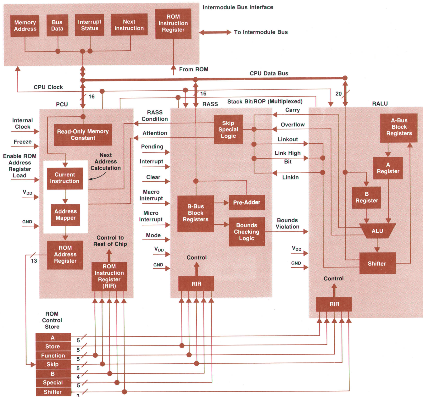
Fig. 3. The HP 300 CPU hardware is functionally partitioned into three CMOS/SOS chips. The processor control unit (PCU) chip generates microinstruction addresses that control the other two chips: the register, address, skip, and special (RASS) chip and the register, arithmetic, and logic unit (RALU) chip.
