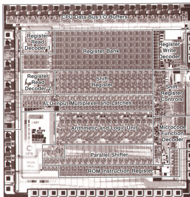
Fig. 7. RALU chip.
