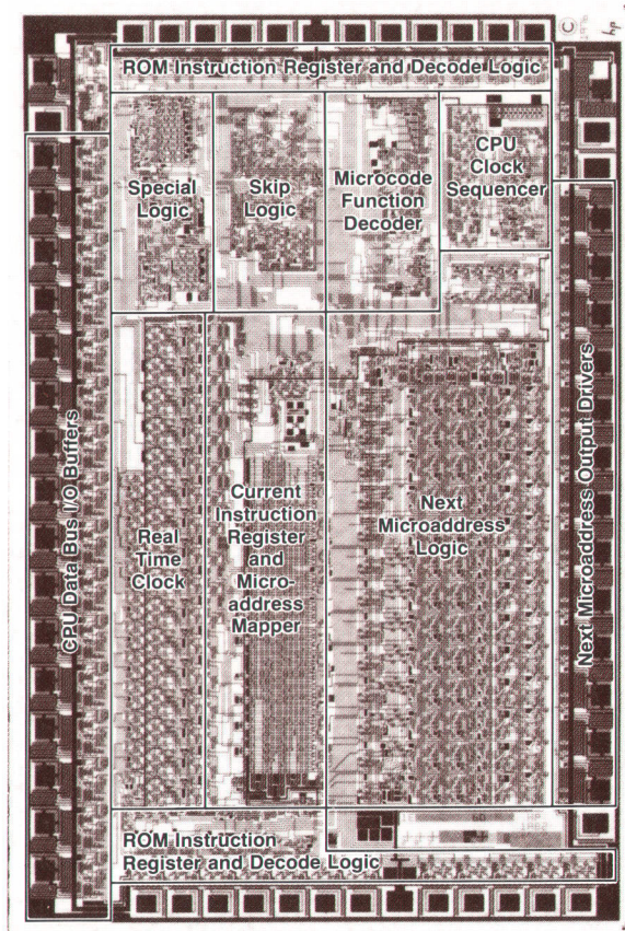
Fig. 5. PCU chip.
