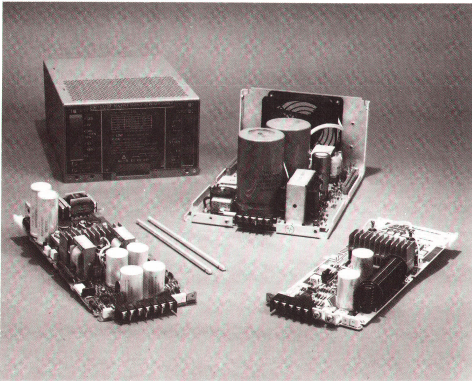
Fig. 1. Three interlocking, functionally independent printed circuit boards contain all the circuits in the 63312F Multiple Output Switching Power Supply. The supply provides up to 550 watts at 5V, \pm 12V or \pm 15V , and up to 40V.
