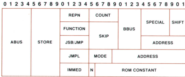
Fig. 8. HP 300 microinstructions are 32 bits wide and come in five formats.
