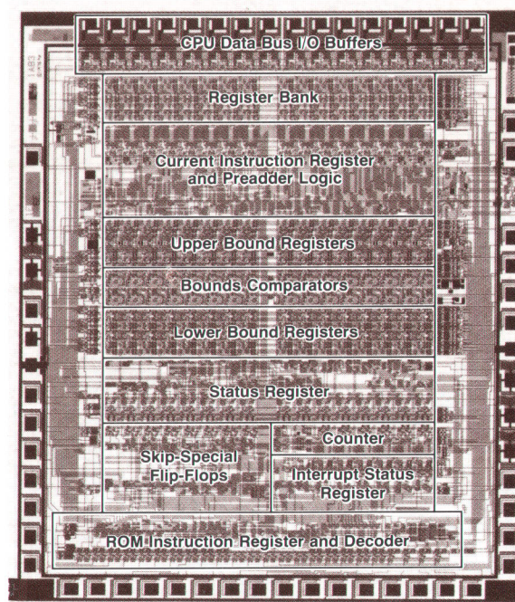
Fig. 6. RASS chip.
