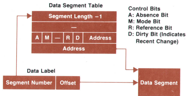
Fig. 2. When variables are passed by reference to a memory location, the pointer to the location is a 32-bit data label that contains a segment number and an offset. The segment number is used to index into the data segment table for the status and location of the segment. Segment presence and mode are checked and the offset is added to the address from the table to give the address of the data.
