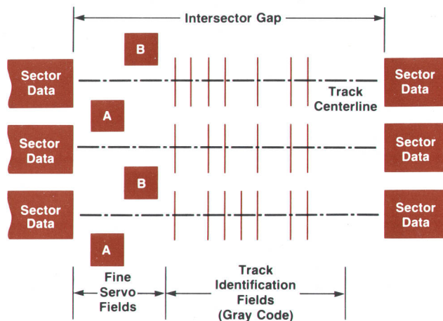
Fig. 2. Information recorded in gaps between data records on the disc makes it possible to use the data surface as a reference for positioning the read/write heads.
