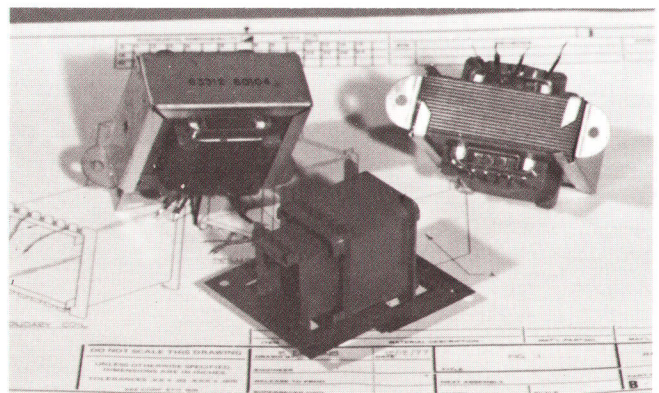
Fig. 5. Bias transformer uses novel concentric bobbins to achieve required safety spacings.
